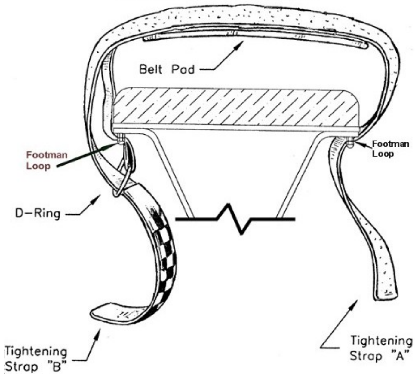
Double Locking Belt Mounting Diagram
